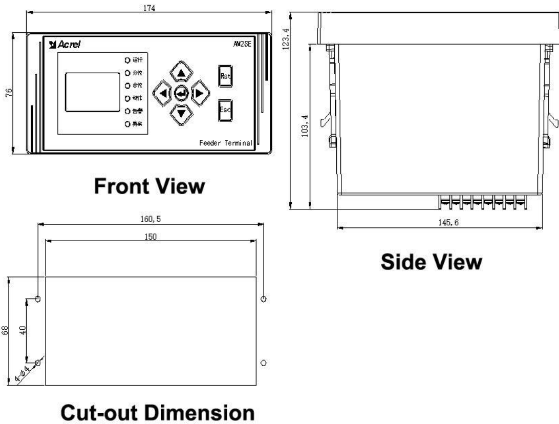
Fig. 4.2 AM2SE-H Dimensions and cut-out dimensions
