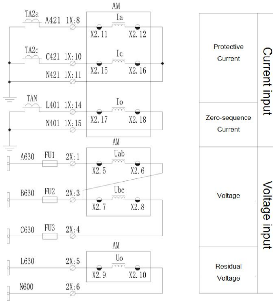
Fig.5.4 2PT & 2CT Wiring
