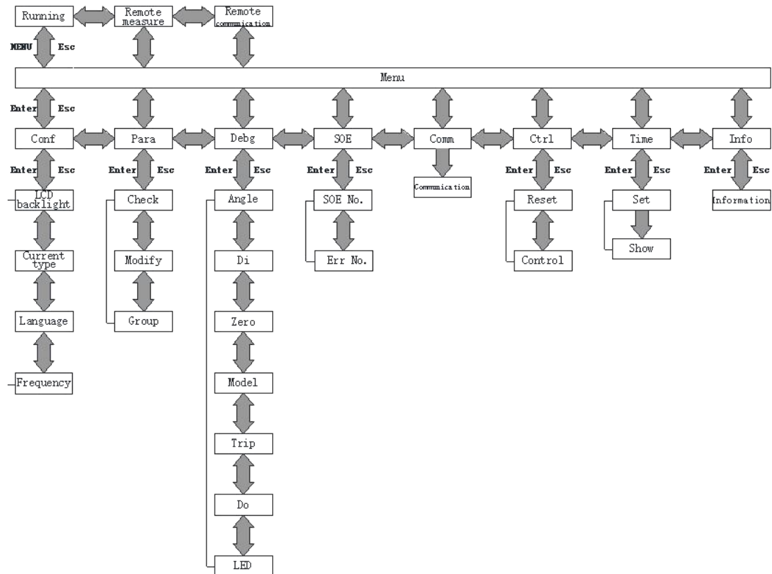
Fig. 3.6 Navigation diagram
