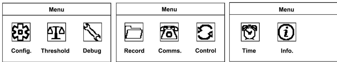
Fig. 3.5 Main Menu
