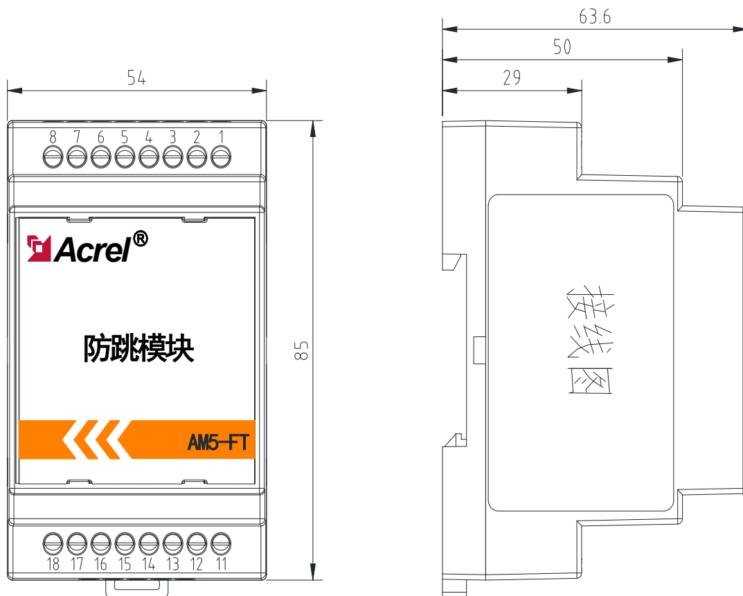
Fig.3 AM5-FT Dimensions
